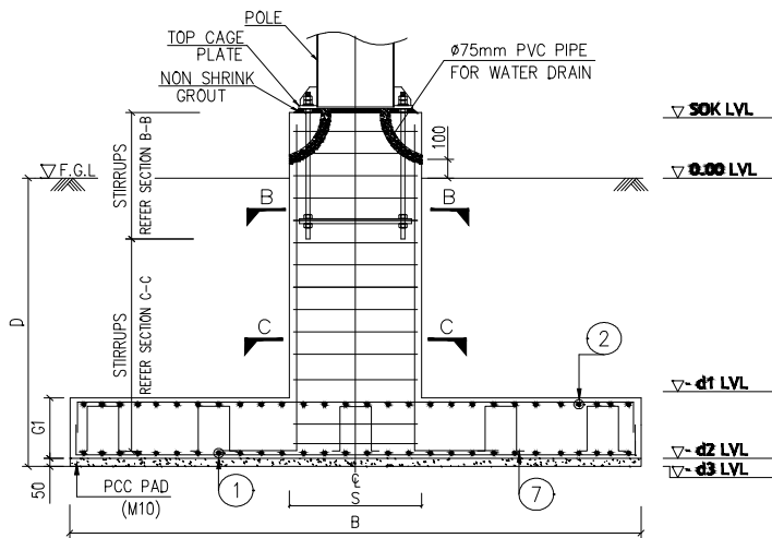
FOUNDATION DETAIL (SECTION "A-A")
