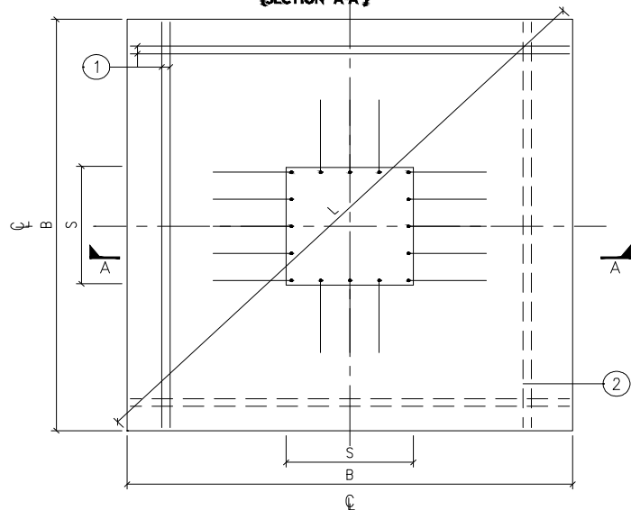
FOUNDATION PLAN (SHOWING BOTTOM & TOP REINFORCEMENT DETAILS)
