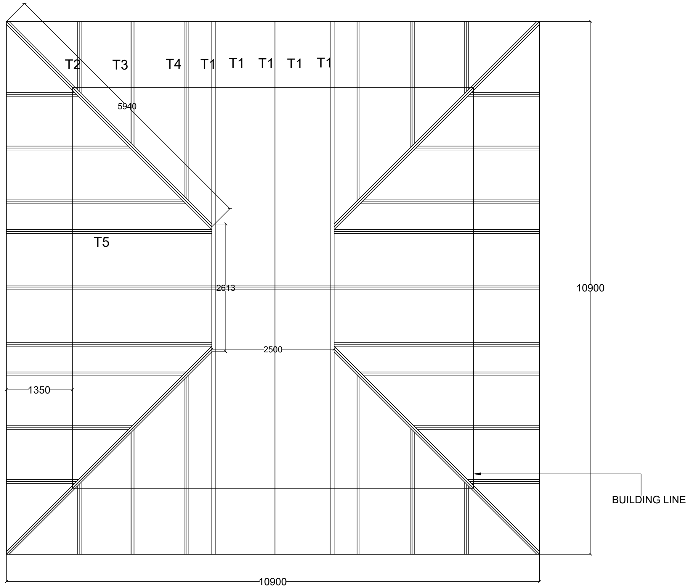
ROOF MEMBER LAYOUT
