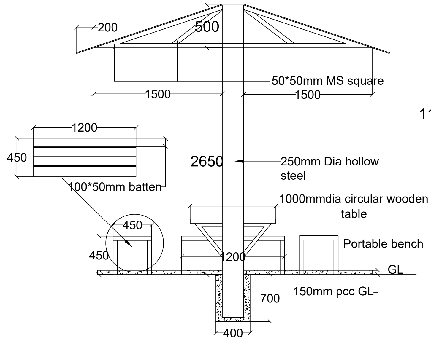
FRONT VIEW
