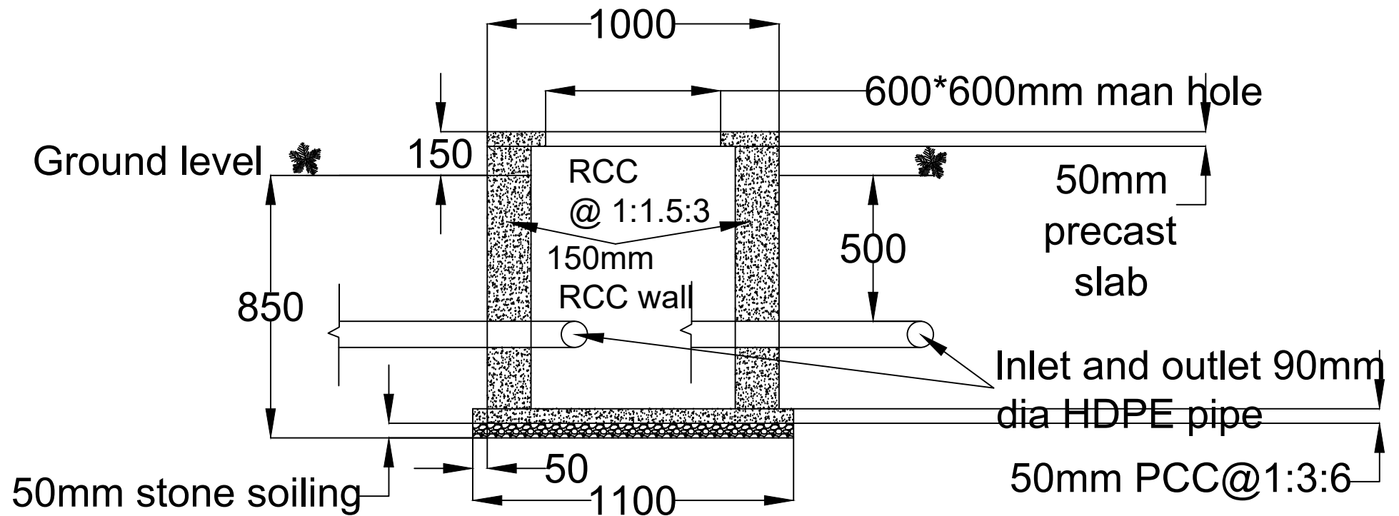
Sectional view of the RCC chamber
