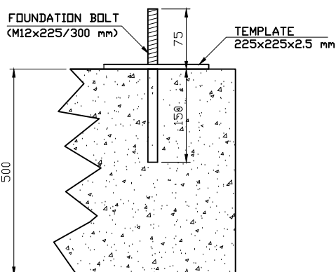
FOUNDATION BOLT INSERTED IN R.C.C. COLUMN
