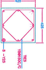
SECTION 2-2
