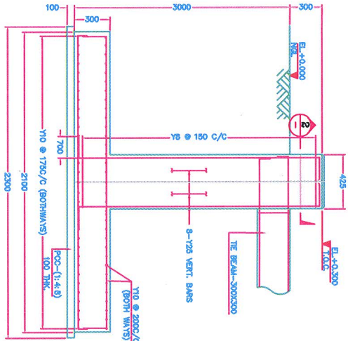
SECTION 1-1
