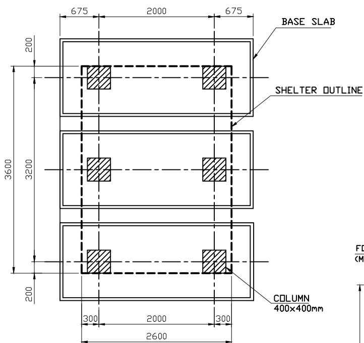
LAYOUT PLAN
