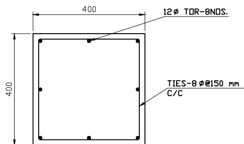
SECTION 'A-A' COLUMN 400x400
