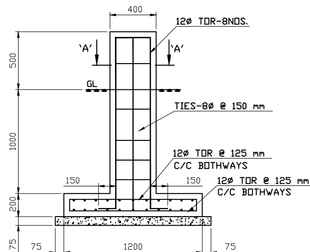
CROSS SECTION (SCALE 2:1)
