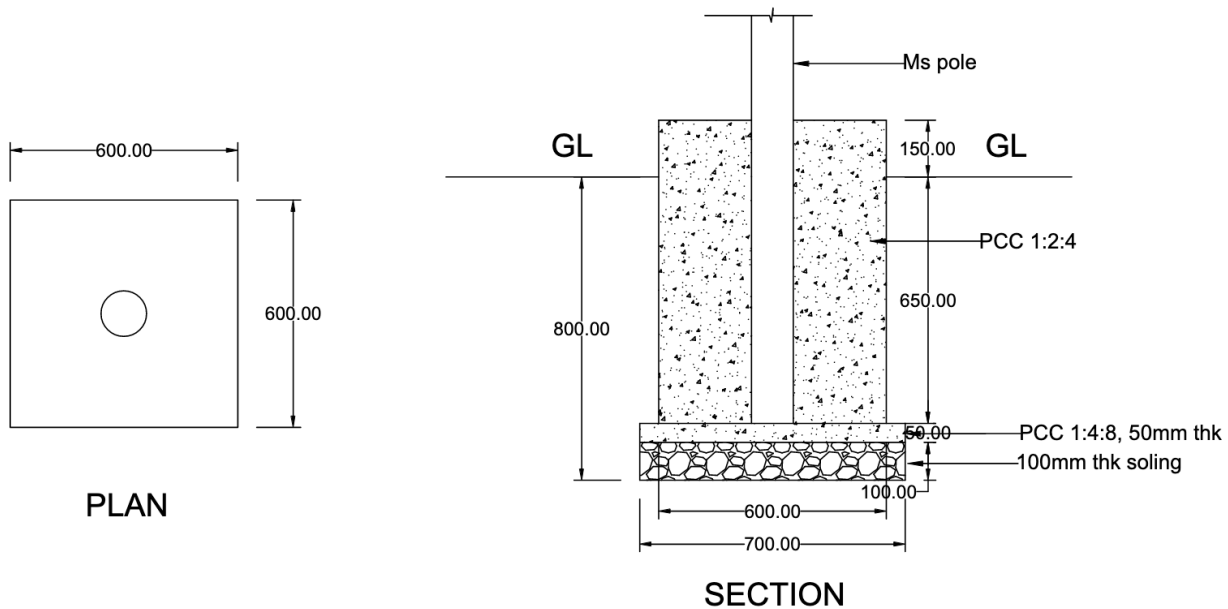
Fig. 1: Drawing for civil foundation works for the lamp post
