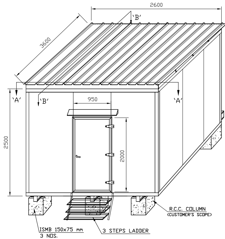
PERSPECTIVE VIEW
