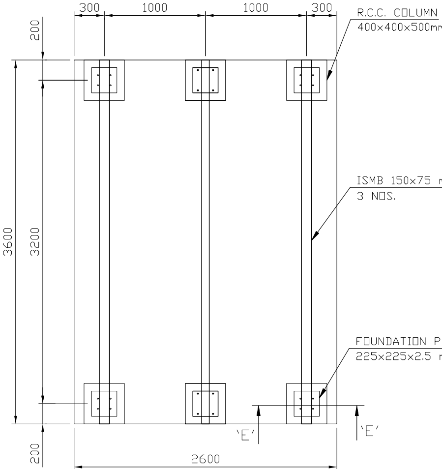
FOUNDATION PLAN
