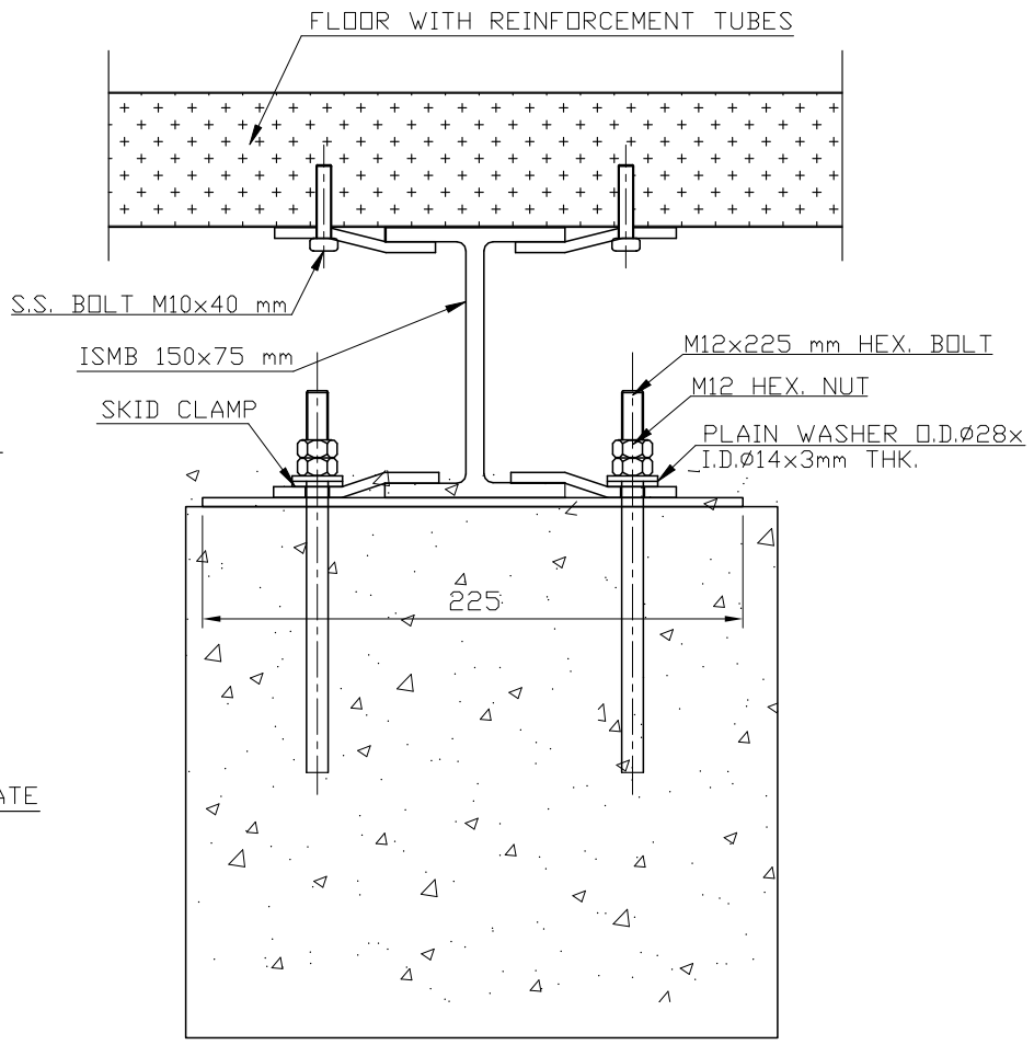
SECTION 'E-E'
