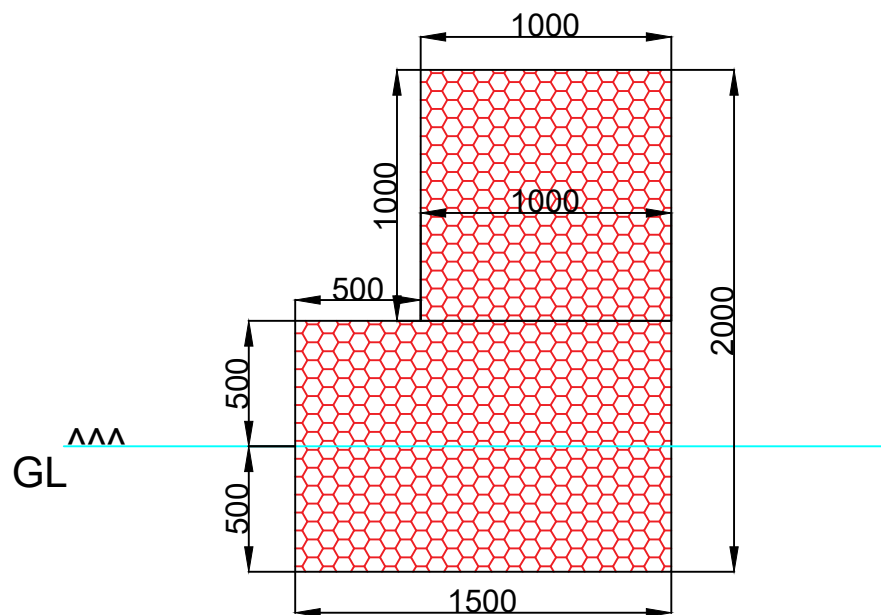
Gabion Wall
