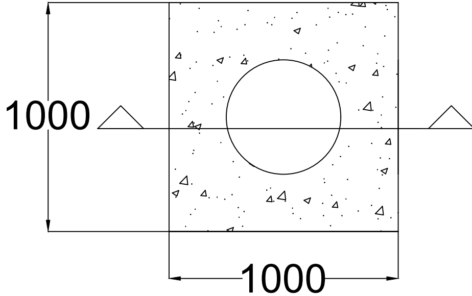
Precast 150mm RCC slab
