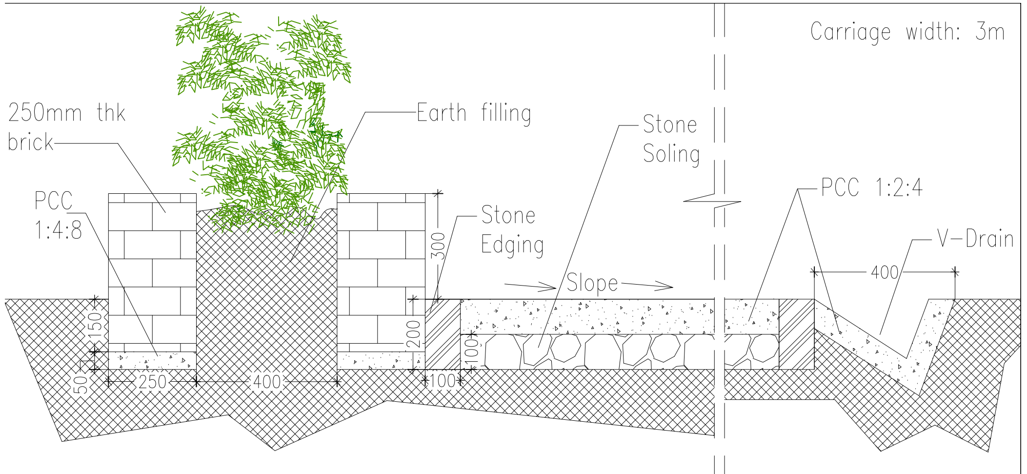
Cross Section of Flower Garden and PCC Pavement
