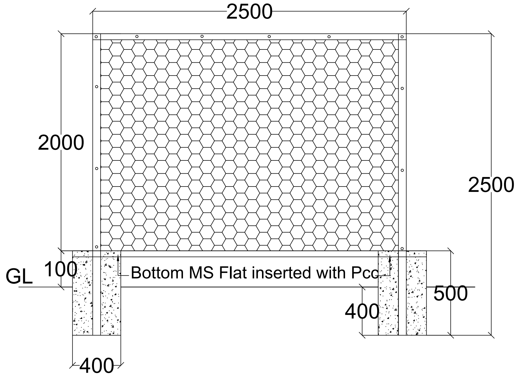
FRONT SECTIONAL VIEW
