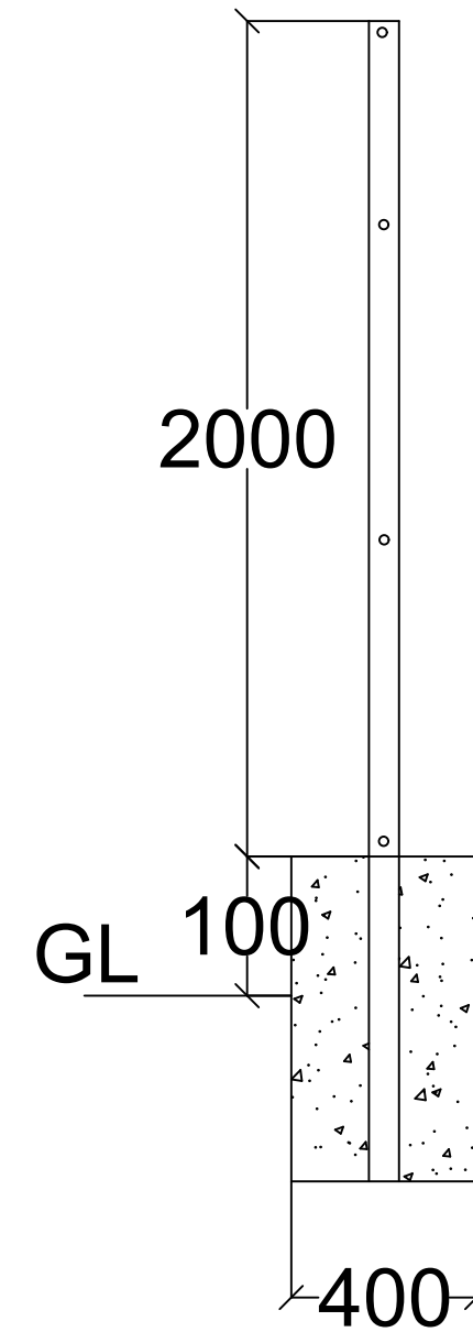
SIDE SECTIONAL VIEW
